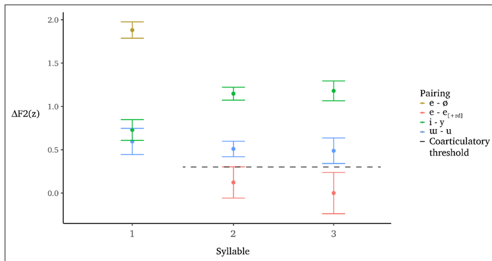
Figure 9: A modified plot of \Delta F2(z) , with 95% confidence intervals) for each vowel pairing and syllable compared to the coarticulatory threshold in Southern Crimean Tatar. All initial-syllable tokens of /y/ following /k g/ were removed, as well as all third-syllable tokens of /i/ where F2(z) > 0 .
